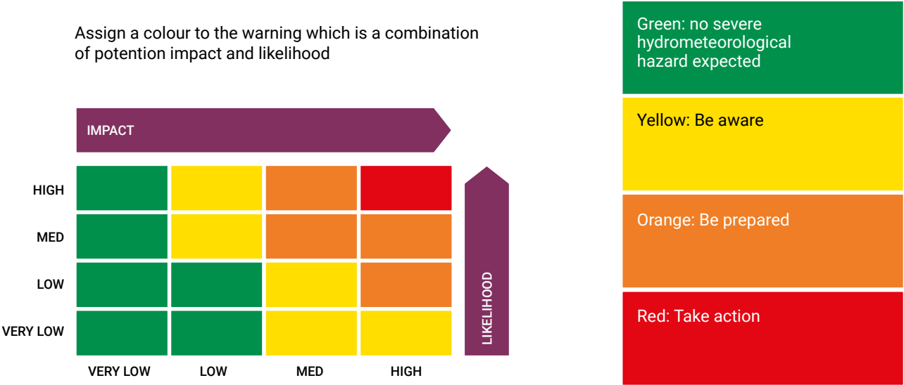
Figure 11 Example of colour-coded risk matrix to derive the severity of warnings. Source: UK Met Office
