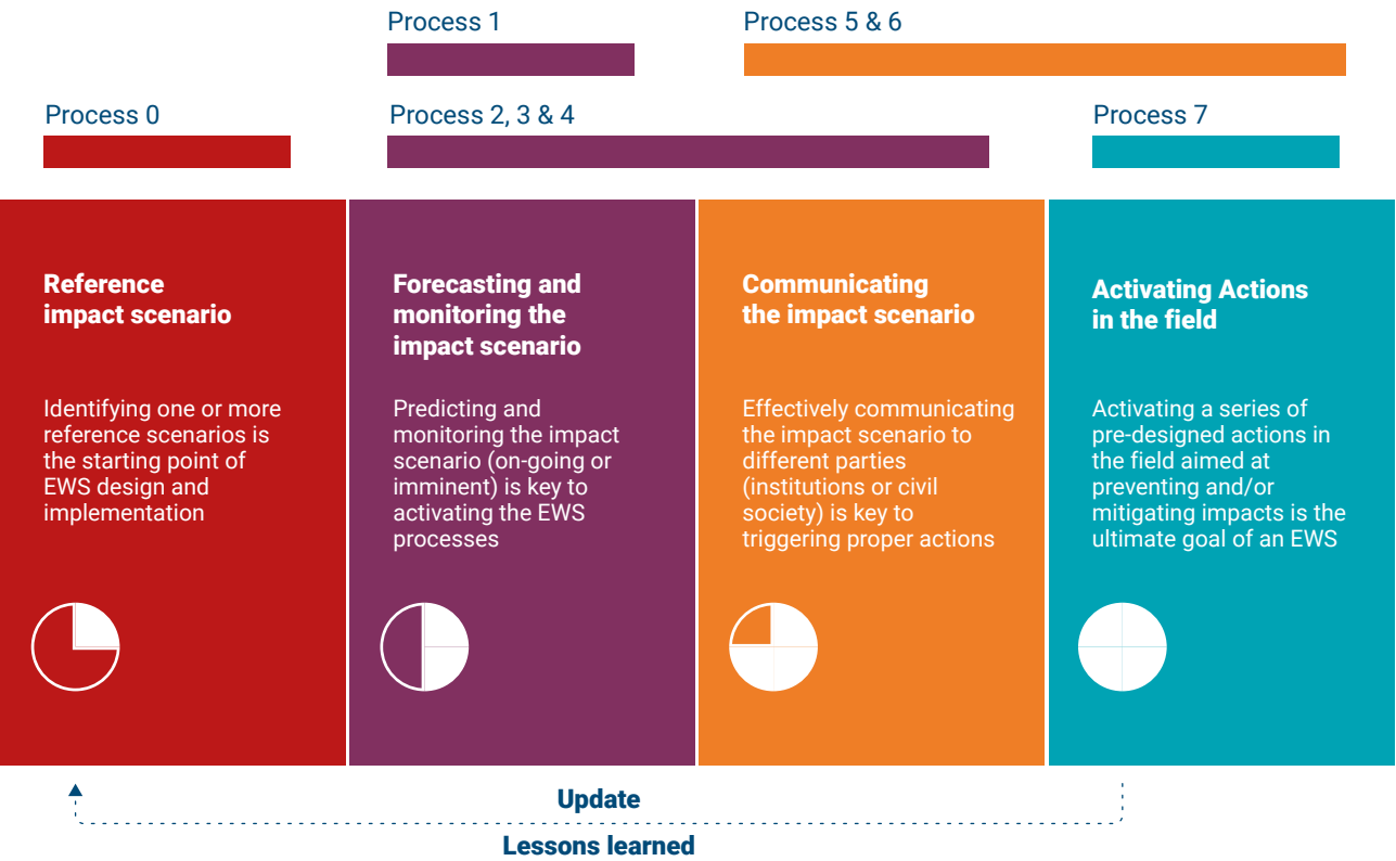
Figure 4 The early warning concept and processes
