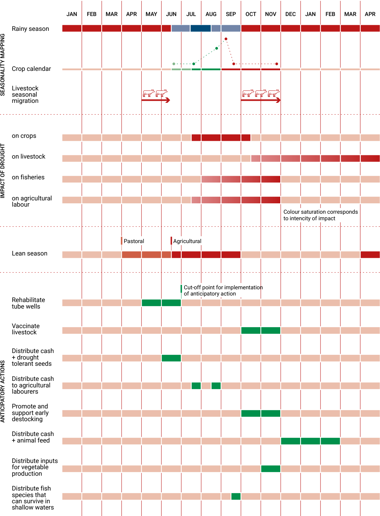
Figure 8 Example of a crisis timeline for drought in an area with a uni-modal rainfall regime with selected anticipatory actions for drought. Source: (FAO, 2022)
