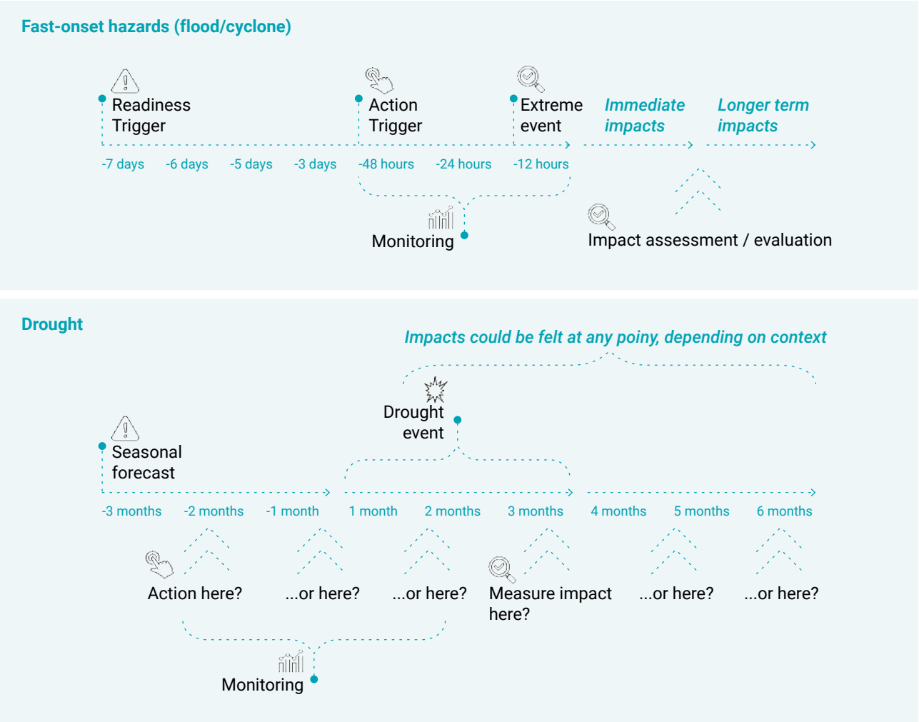
Figure 14 Differences in timelines between fast-onset hazards (flood/ cyclone) and droughts (WFP, 2021)
