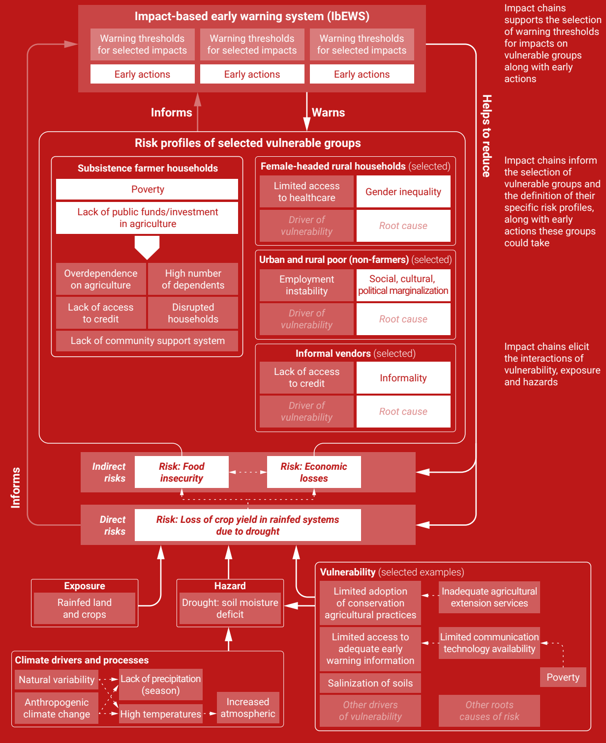
Figure 9 Impact chain to support IBF and IbEW. Through selected examples, the figure shows a simplified version of the interconnections of drivers of risks and risk profiles for direct (“Loss of crop yield in rainfed systems due to drought”) and indirect risks (“Food insecurity”, “Economic losses”) in Kenya. The model also illustrates how impact-based warning and early actions can be informed by and subsequently help reduce these risks.
