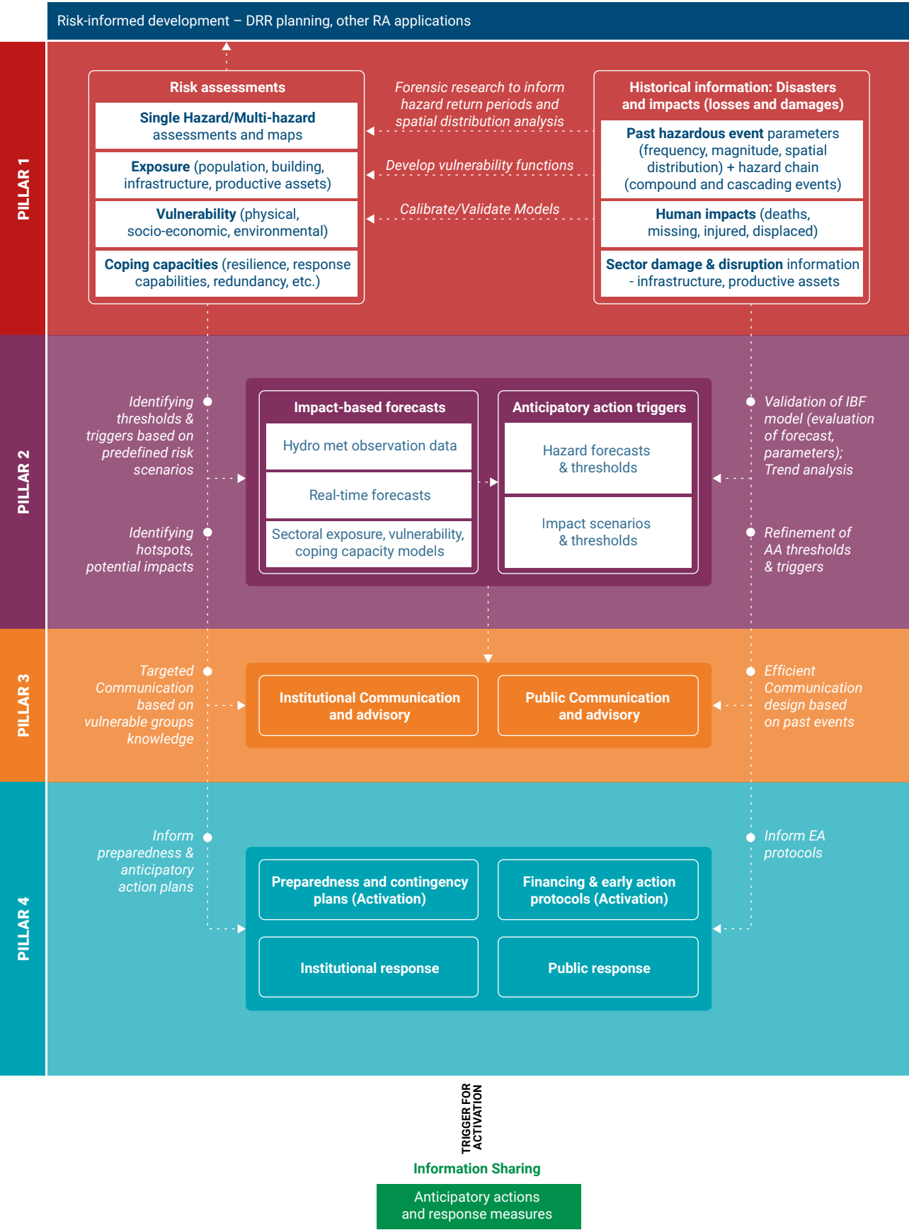
Figure 2 The importance of risk knowledge (assembled from historical disaster loss and damage information) for the EW4All pillars and development of impact-based forecasts and anticipatory actions (modified by UNDRR)
