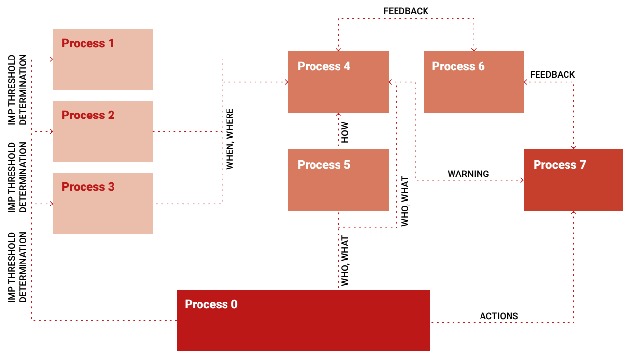
Figure 7 Risk information for EWS: workflow, processes and linkages
