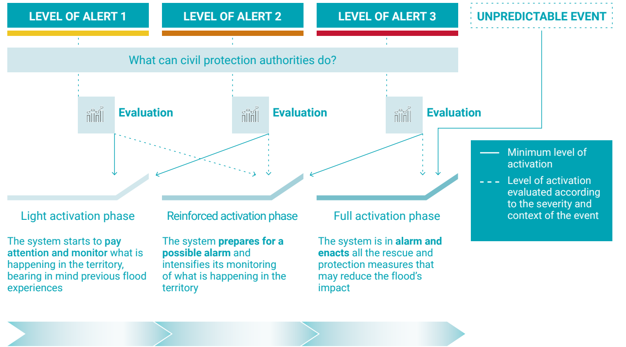
Figure 15 Increasing activation phases of the civil protection system and related early actions for floods. Source: (Giambelli et al., 2023)
