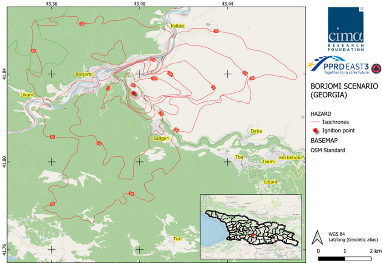
Figure 10 Example of a risk scenario development
