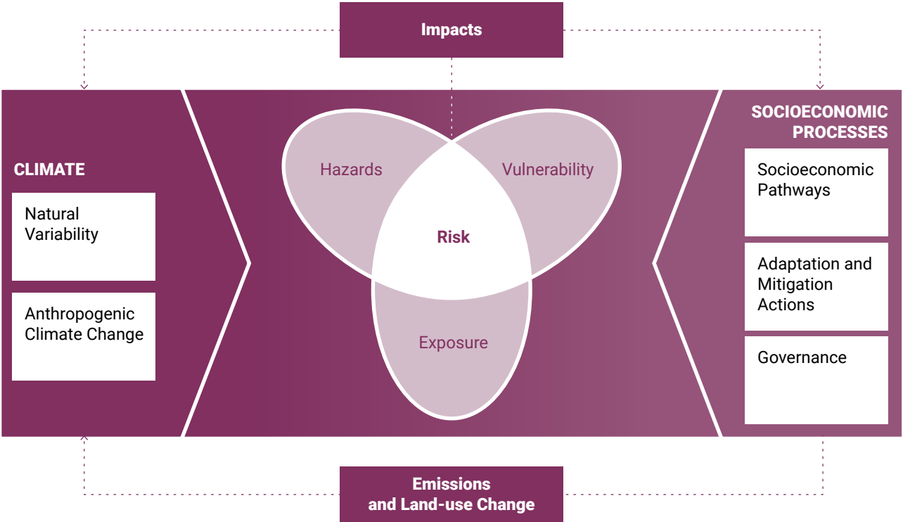
Figure 12 The IPCC AR5 conceptual risk assessment framework (IPCC, 2014)
