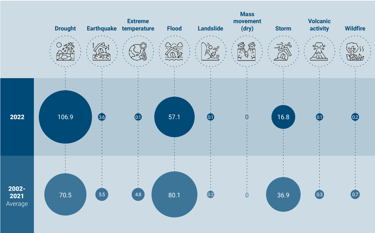
Figure 1 Number of people affected (million) by disaster type: 2022 compared to the 2002-2021 annual average
