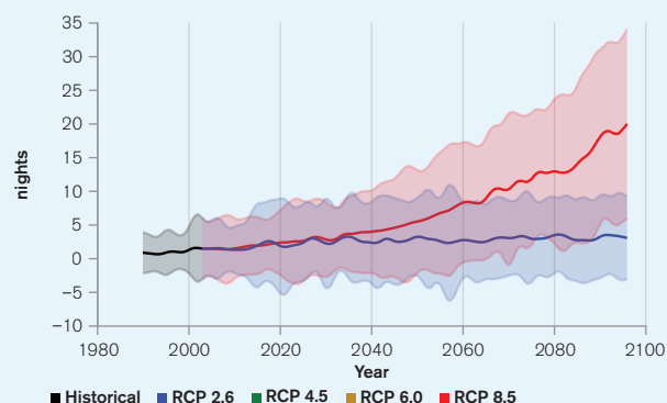
FIGURE 13. The historical and projected number of Tropical Nights (Tmin >20°C) through the end of the century
