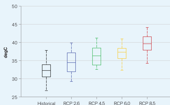
FIGURE 11. Average daily maximum temperature in Georgia under four emissions pathways over the period 2080–2099.
