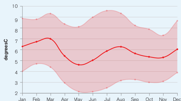
FIGURE 7. Projected change (°C) in monthly temperature, shown by month, for Kazakhstan for the period 2080–2099 under RCP8.5. The value shown represents the median of the model ensemble with the shaded areas showing the 10th–90th percentiles. 21
