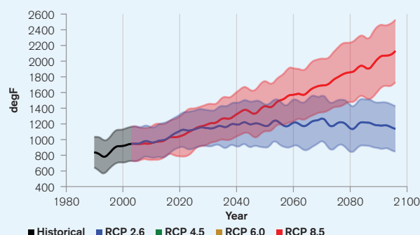
FIGURE 11. Historical and projected annual cooling degree days in Kazakhstan (cumulative degrees above 65°F) under RCP2.6 (blue) and RCP8.5 (red). The values shown represent the median of 30+ GCM model ensemble with the shaded areas showing the 10–90th percentiles 21 .
