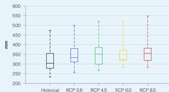
FIGURE 8. Projected average annual precipitation (mm) for Kazakhstan in the period 2080–2099. 21
