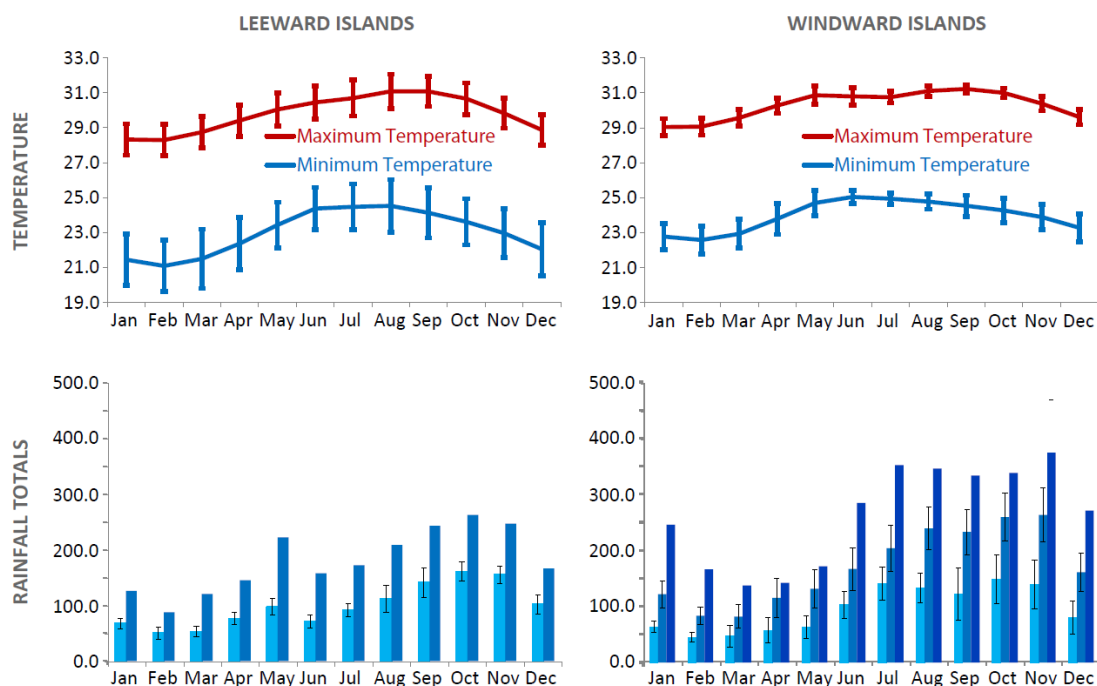
Figure 1 Climatology of the seasonality of maximum temperature, minimum temperature (top panels) and rainfall totals (bottom panels) across the Leeward Islands (left panels) and Windward Islands (right panels) of the OECS region.
