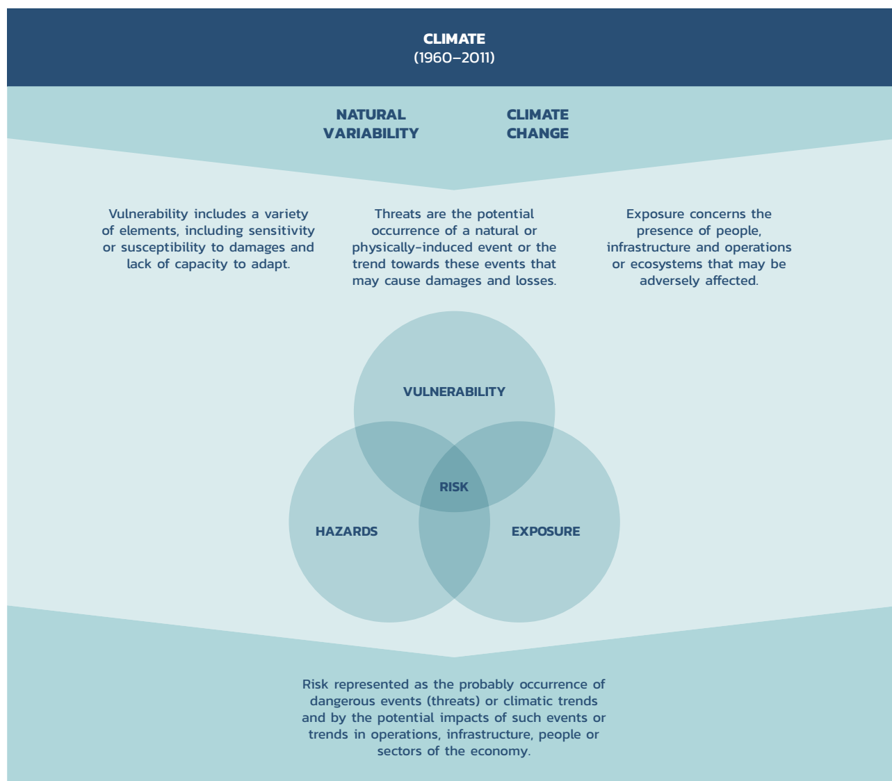
Figure 3: Climate Risk Analysis Methodology.
