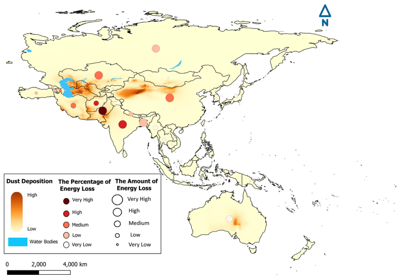
Figure 3-10: The amount of energy loss and percentage of energy loss in energy production of the solar powerplant in Asia-Pacific countries
