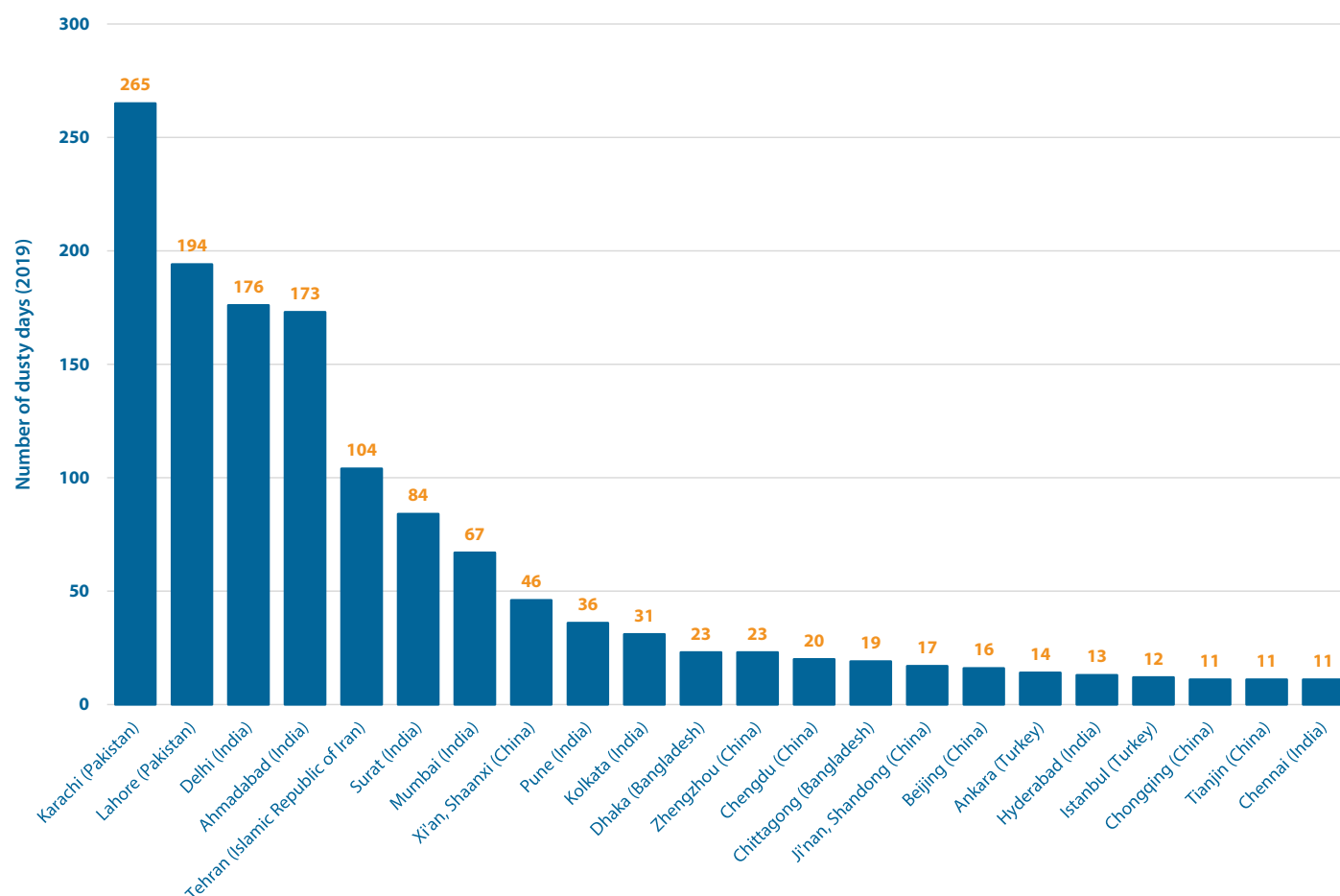
Figure 3-7: Big cities (population more than 5 million) with the highest number of days that the amount of dust exceeds 50 \mu g/m 3 annually
