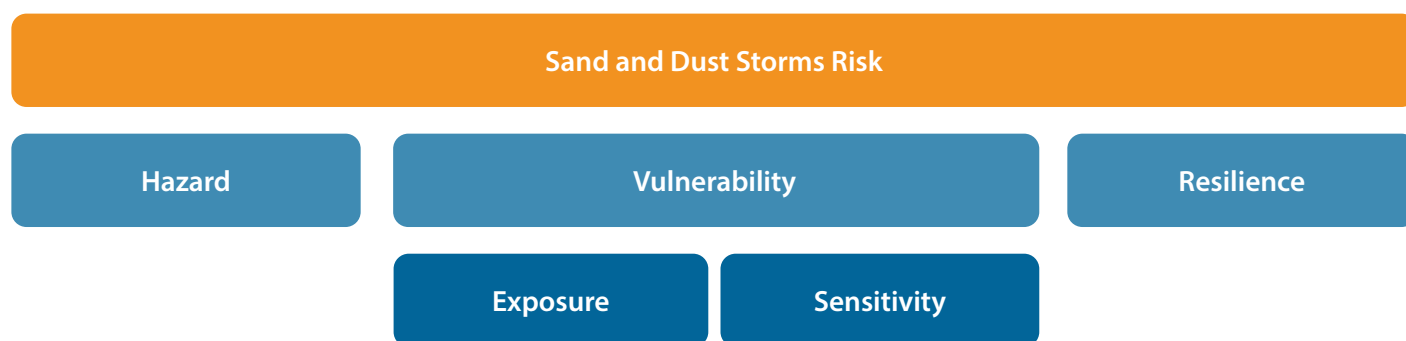
Figure 2-1: Conceptual framework of the sand and dust storms risk assessment
