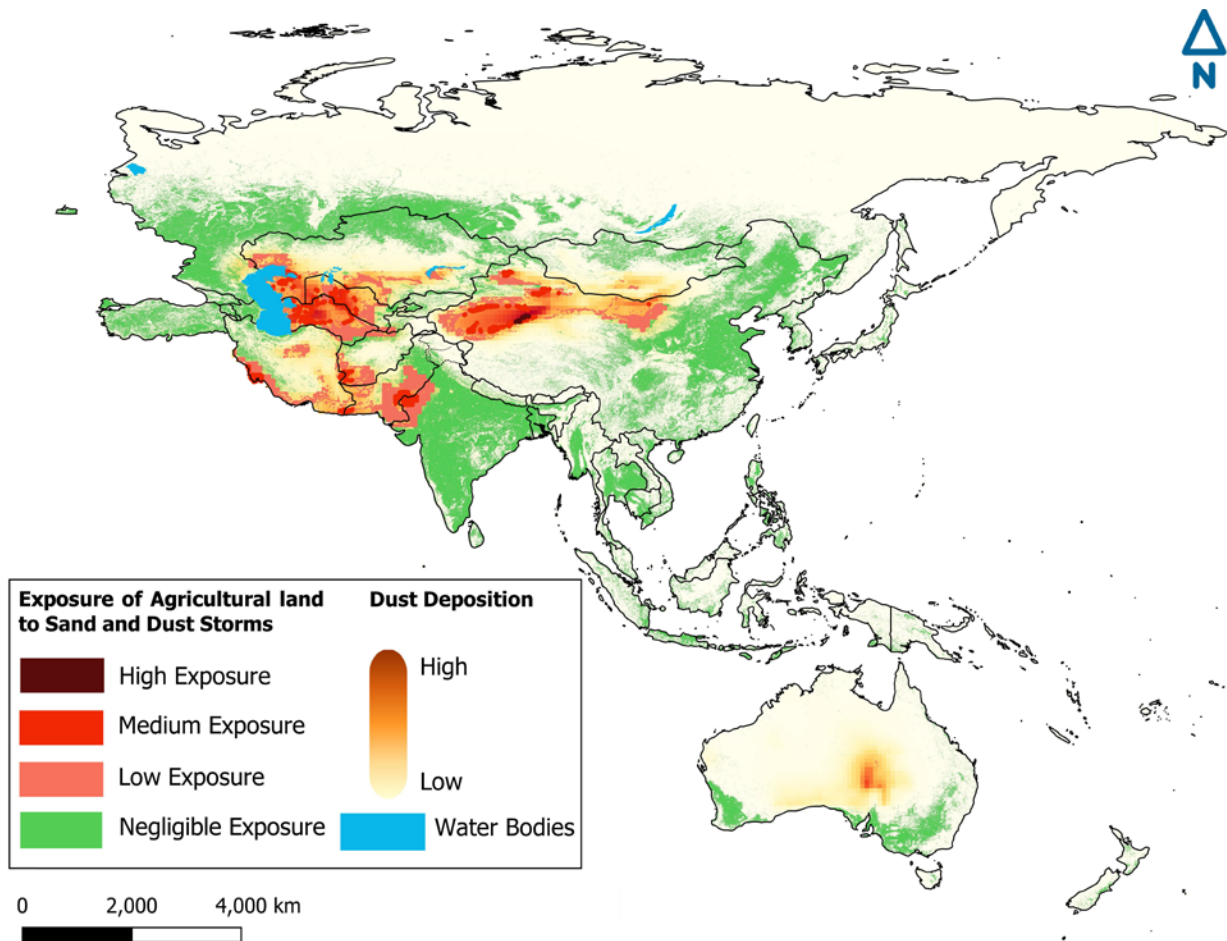
Figure 3-19: The exposure of agricultural land to average dust deposition (2019)
