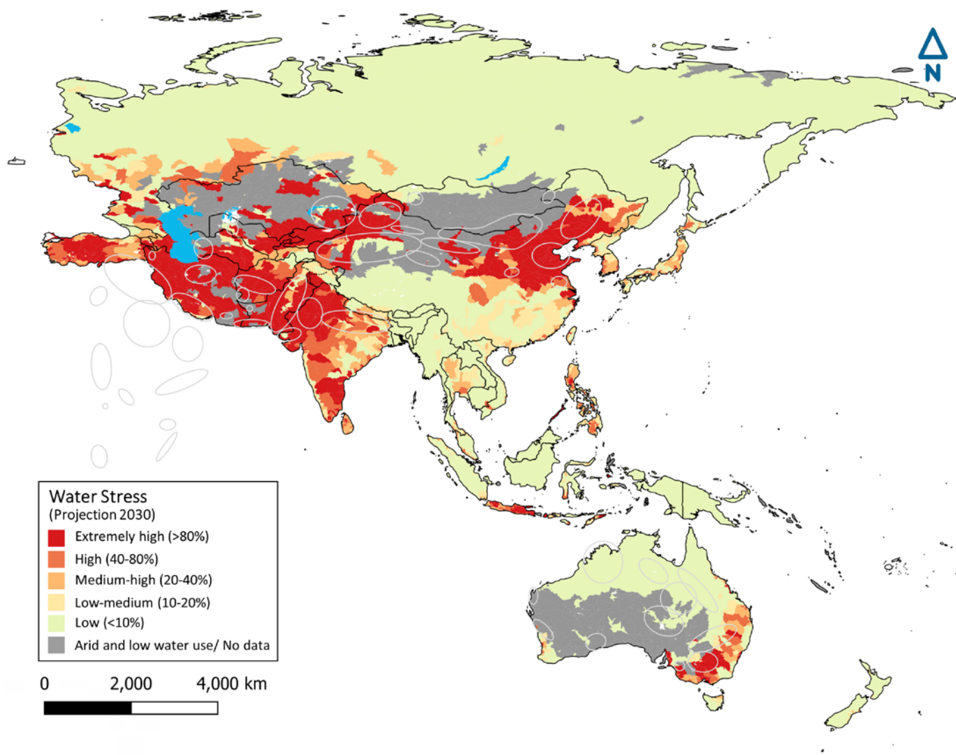
Figure 4-3: Water stress (Projection 2030)
