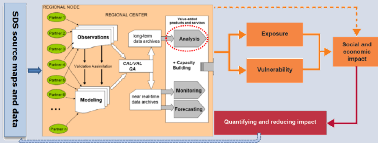
Figure 5-3: Scheme of SDS-WAS regional center's long-term SDS impact assessments **
