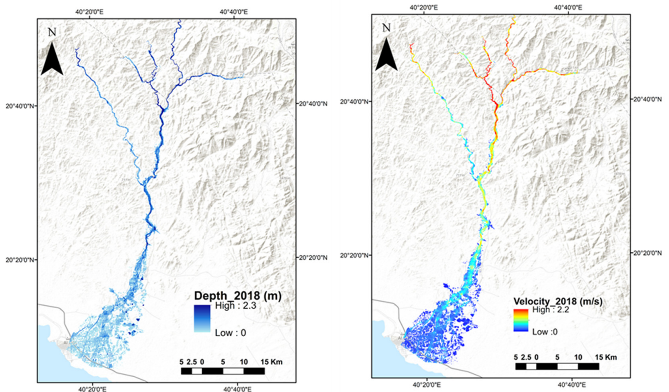
Figure 8. Flood water velocity and depth map of the Al-Lith Valley Basin impacting Al-Lith City in 2018.
