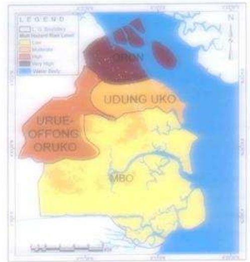
Fig. 4 Multi Hazard Risk Zones of the study area
