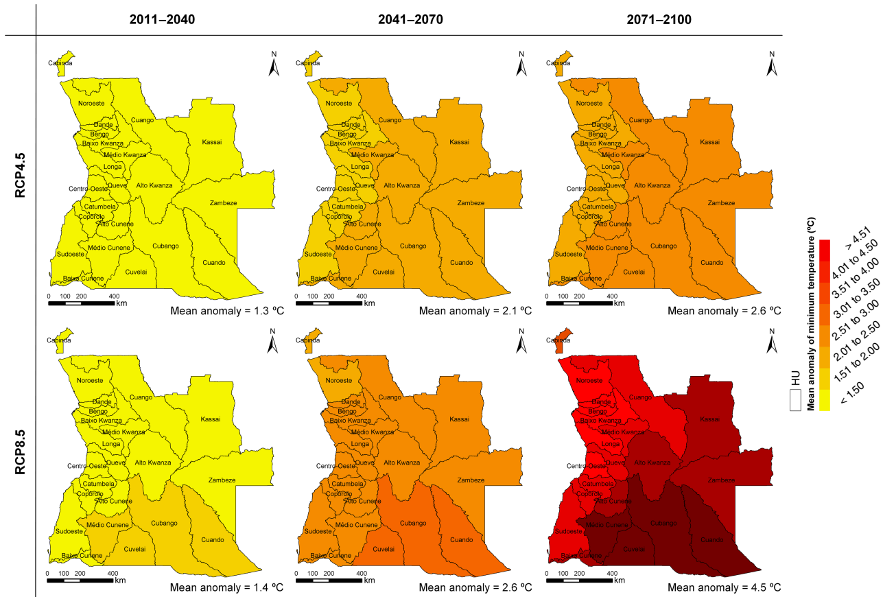
Figure 5. Mean anomaly of minimum temperature for the three time periods and two RCPs based on the RCMs ensemble.
