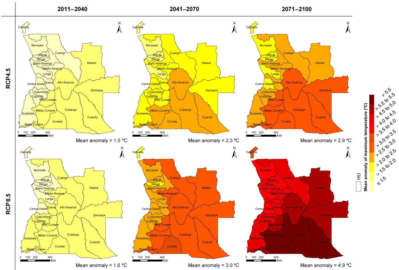
Figure 4. Mean anomaly of maximum temperature for the three time periods and two RCPs based on the RCMs ensemble.
