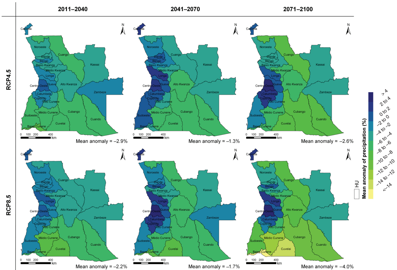
Figure 7. Mean anomaly of precipitation for the three time periods and two RCPs based on the RCMs ensemble.
