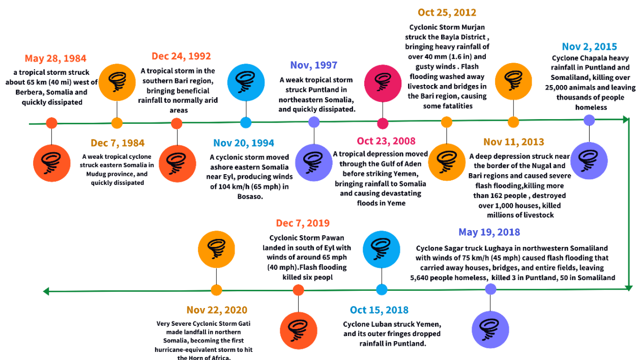
Figure 4 : Track record of cyclonic landfall over the Somalian coast from 1984-2020, Source: Wikipedia 2024
