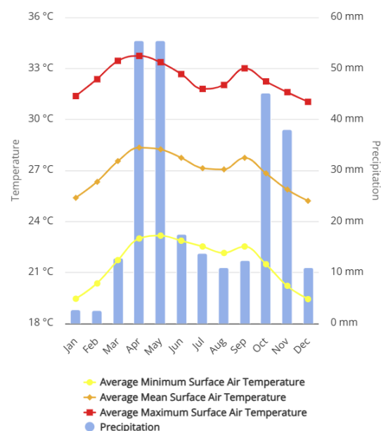
Figure 8: Monthly climatology of average minimum surface air temperature, average mean surface temperature, average maximum surface temperature & precipitation 1991-2022 Somalia 3
