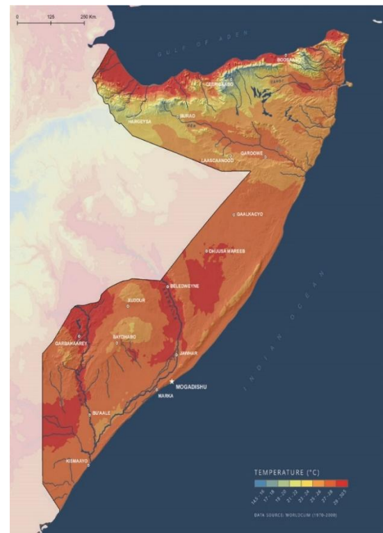
Figure 3: Average temperature Source: Original calculations based on TerraClimate
